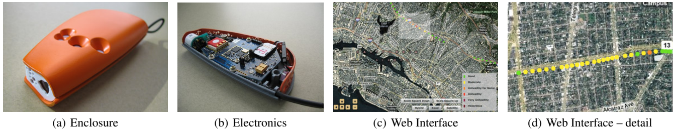
Figure 1. The current hardware can be selectively populated with commercial carbon monoxide, nitrogen oxides, and ozone gas sensors as well as light, temperature, relative humidity, and orientation sensors. This sensor data is acquired and processed locally using the Epic Core module [3], which also provides an 802.15.4 interface suitable for connecting with other sensors or low-power networks. The handheld monitor can be tethered to a mobile phone using the handheld's integrated BlueSmiRF Bluetooth module from SparkFun which allows sensor readings to be easily visualized on a mobile phone. Finally, a Cinterion GPRS radio and GPS receiver enable the sensor samples to be space-time stamped and uploaded to a hosted server for dissemination, visualization, and analysis over the web. Photos (a) and (b) by Mazzarello Media and Arts.
